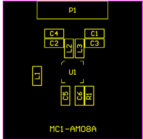
MC1-AM08A Assembly Drawing
