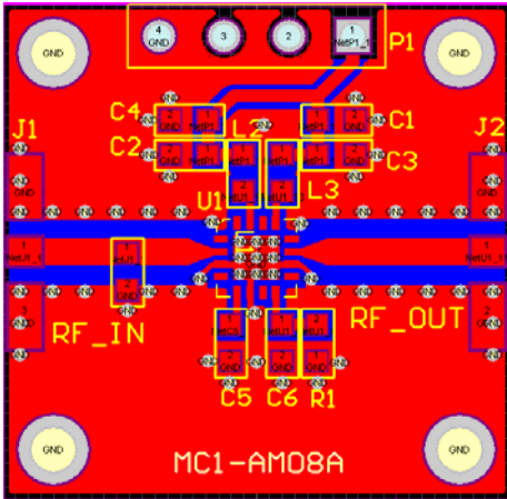
MC1-AM08A PCB Layout:
