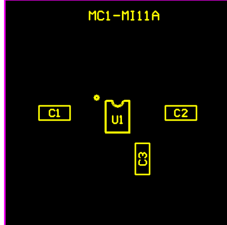
MC1-MI11A Assembly Drawing:
